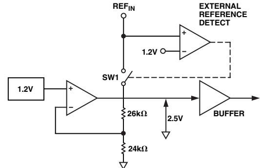
Figure 4. On-Chip Reference
