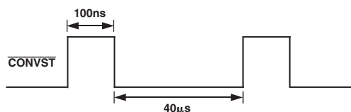
Figure 17. \overline{\text{CONVST}} When Temperature Channel Selected
