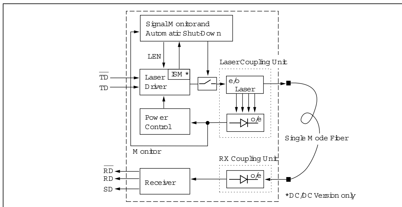
Figure 2 Functional Diagram
