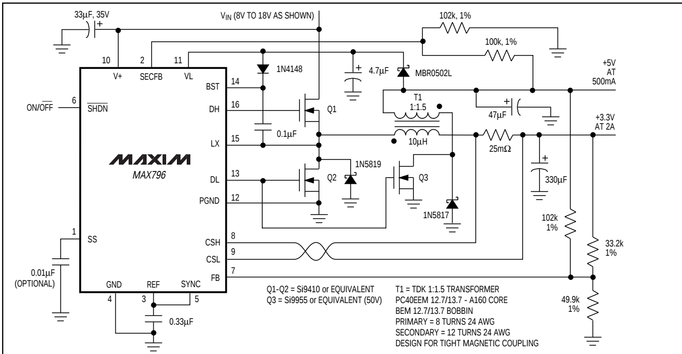
Figure 12. +3.3V/+5V Dual-Output Application (MAX796)
