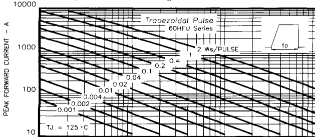
Fig.2 - Maximum Forward Energy Loss Per Pulse Characteristics
