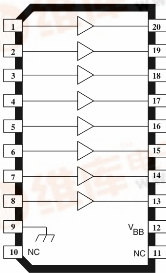
Dwg. PP-064-3
