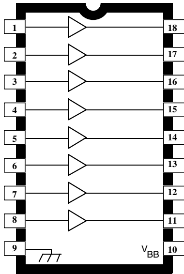
Dwg. PP-065
