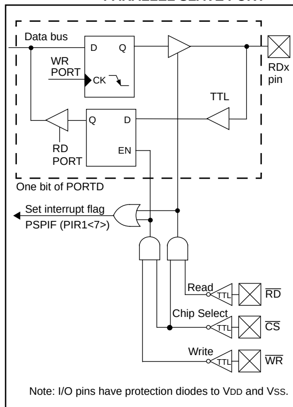
FIGURE 5-12: PORTD AND PORTE AS A PARALLEL SLAVE PORT
