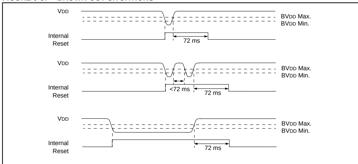
FIGURE 9-8: BROWN-OUT SITUATIONS
