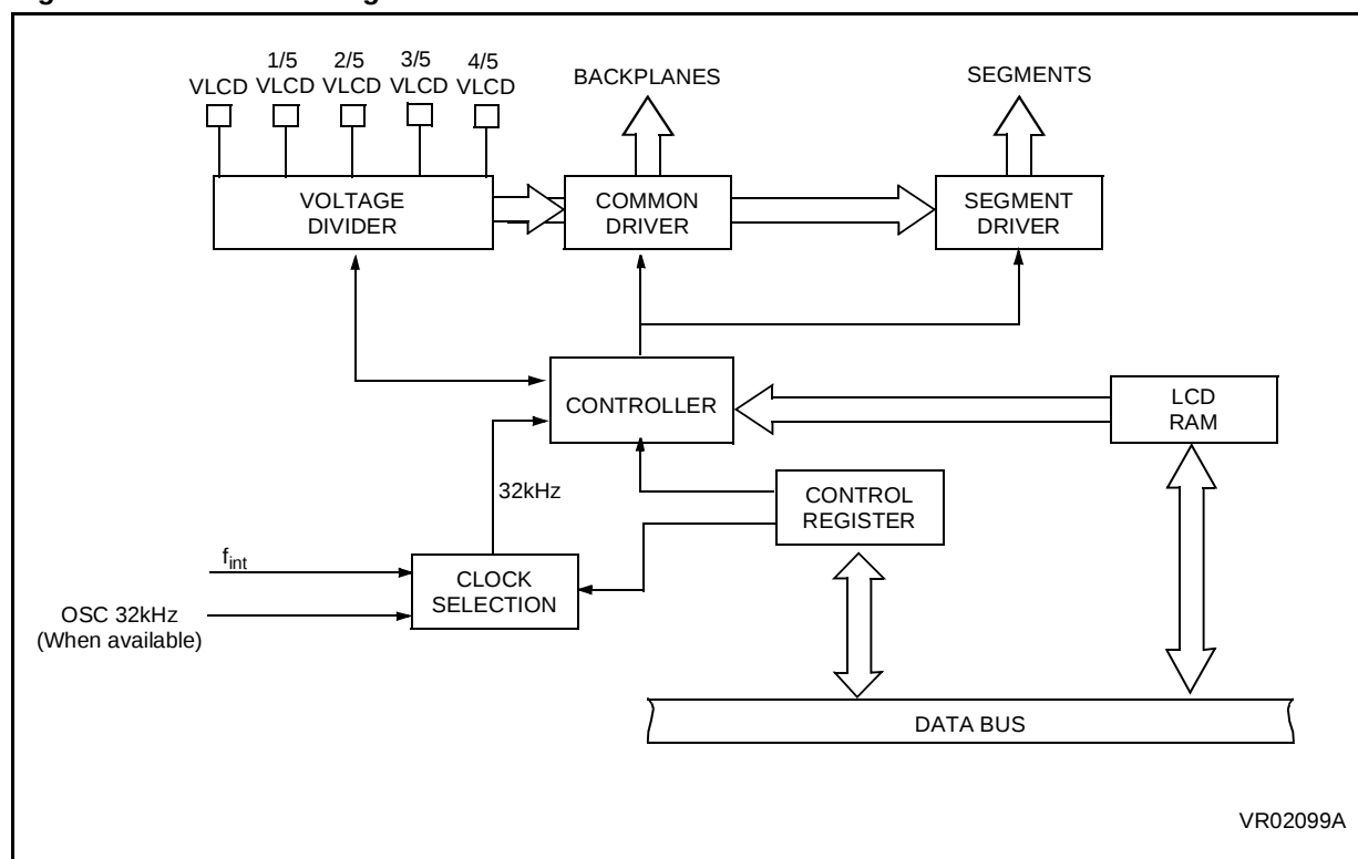
Figure 31. LCD Block Diagram
