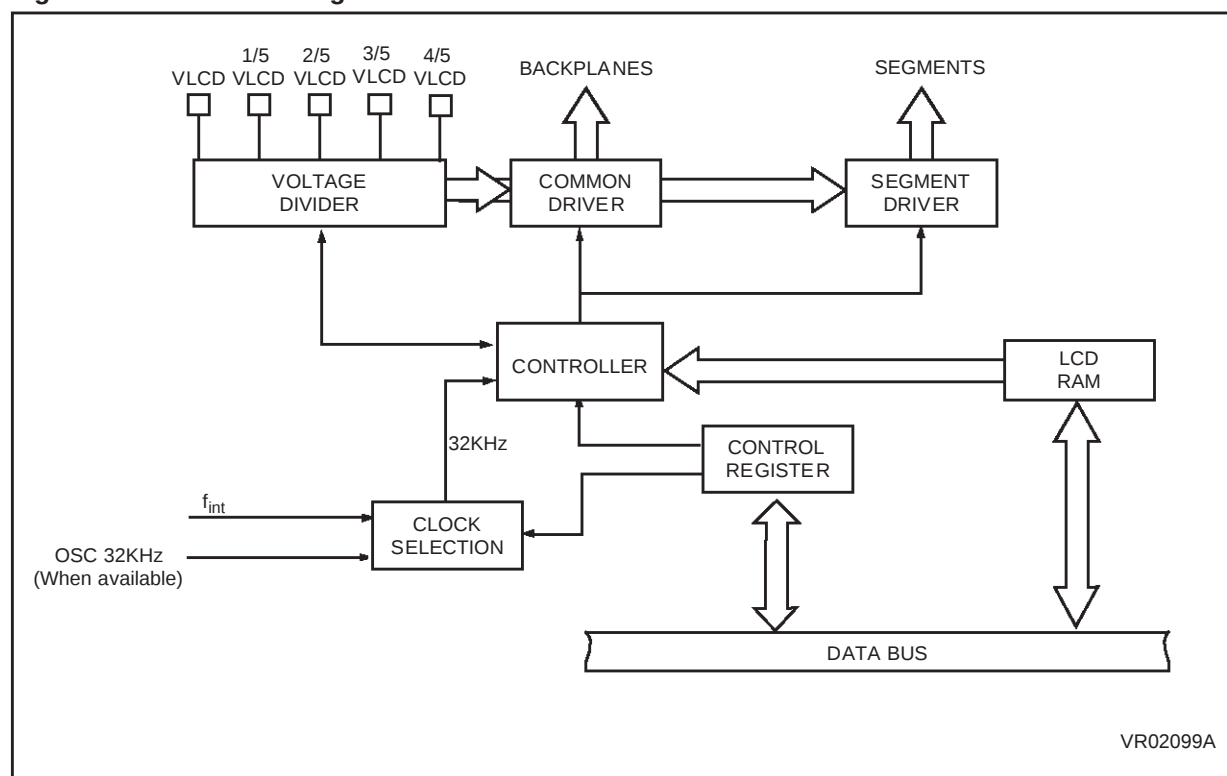
Figure 29. LCD Block Diagram
