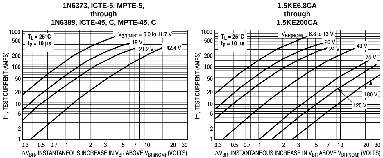
Figure 6. Dynamic Impedance
