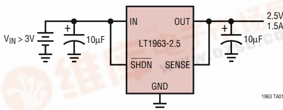
3.3V to 2.5V Regulator
