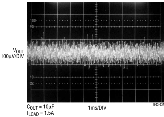
LT1963-3.3 10Hz to 100kHz Output Noise
