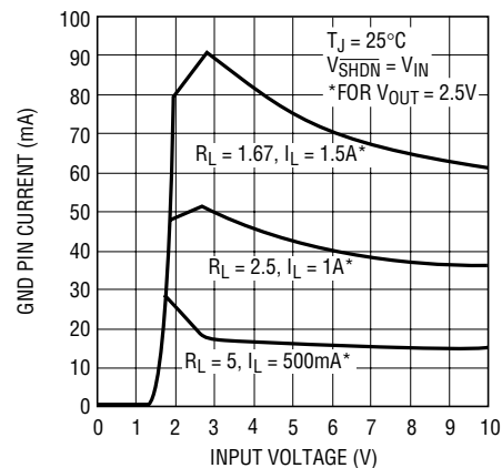
LT1963-2.5 GND Pin Current
