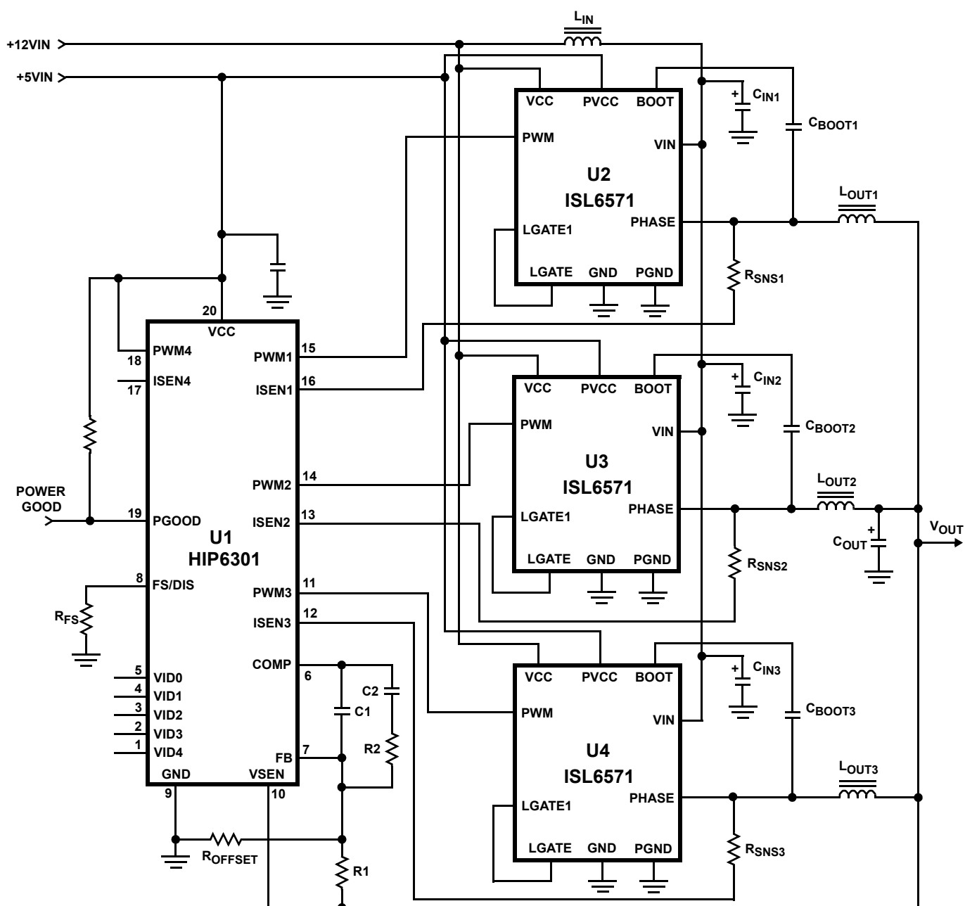
FIGURE 3. TYPICAL APPLICATION
