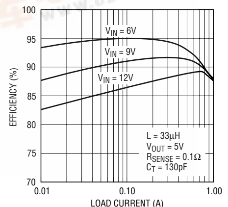
LTC1265-5 Efficiency
