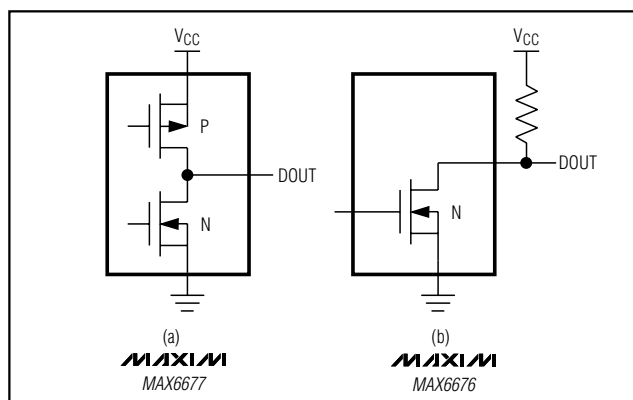
Figure 2. Output Configurations
