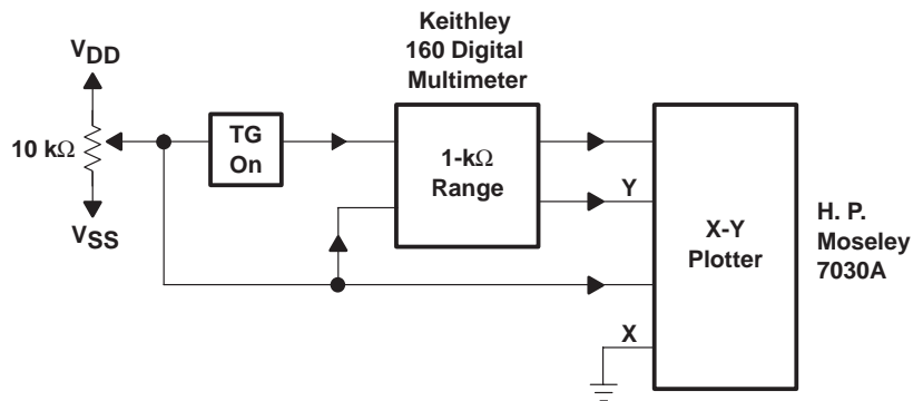
Figure 6. Determination of r_{on} as a Test Condition for Control-Input High-Voltage ( V_{IHC} ) Specification
