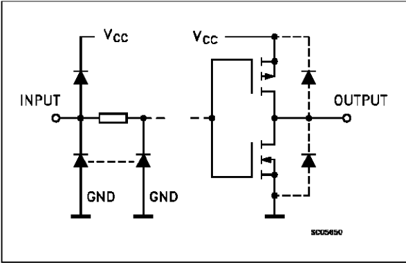
INPUT AND OUTPUT EQUIVALENT CIRCUIT (HC7266)
