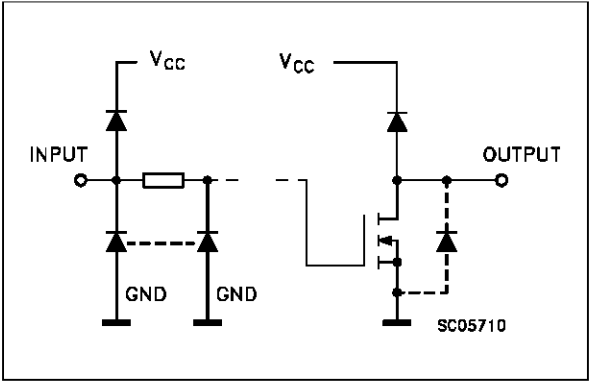
INPUT AND OUTPUT EQUIVALENT CIRCUIT (HC266)
