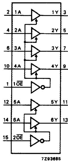
Fig.4 Functional diagram.
