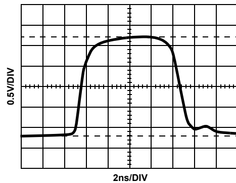
FIGURE 6. RISE AND FALL TIME (6-PIN SOT-23)
