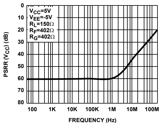
FIGURE 11. PSRR +5V
