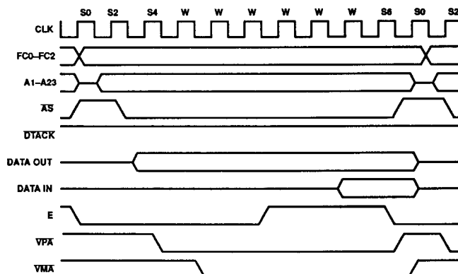
Figure 39. 68000 to Synchronous Peripheral Timing — Best Case
