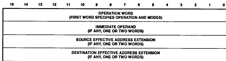
Figure 6. Instruction Operation Word General Format
