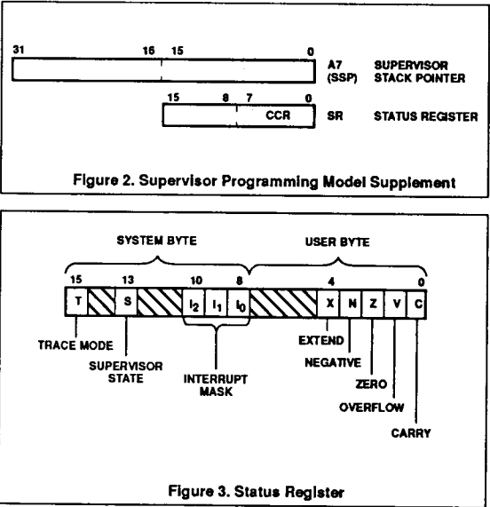
Figure 3. Status Register
