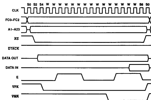
Figure 39. 68000 to Synchronous Peripheral Timing — Worst Case
