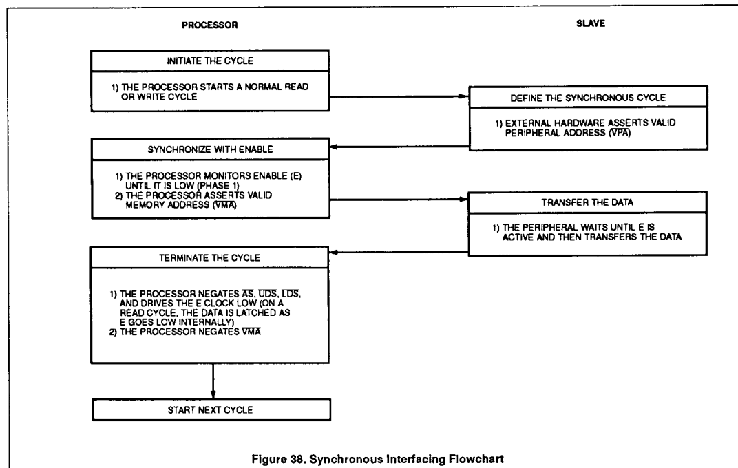
Figure 38. Synchronous Interfacing Flowchart
