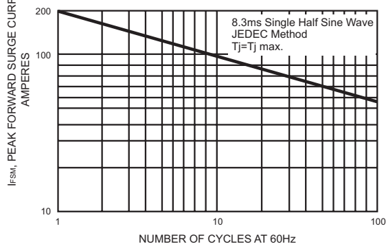
FIG.5- MAXIMUM NON-REPETITIVE FORWARD SURGE CURRENT UNIDIRECTIONAL ONLY
