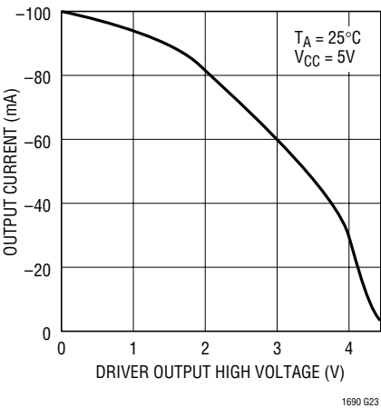
Driver Output High Voltage vs Output Current
