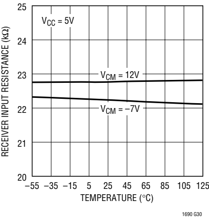
Receiver Input Resistance vs Temperature
