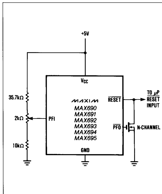
Figure 10. Reset on Overvoltage or Undervoltage
