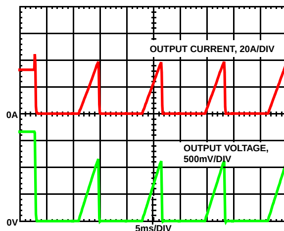
FIGURE 12. OVERCURRENT BEHAVIOR IN HICUP MODE
