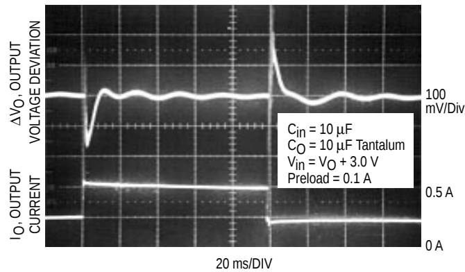
Figure 2. Transient Load Regulation
