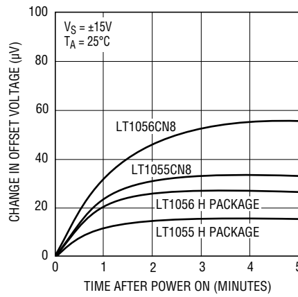
Warm-Up Drift
