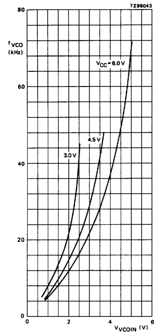
(b) R_1 = 3 \text{ k}\Omega ; C_1 = 100 \text{ nF}
