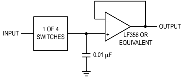
Figure 21. Sample/Hold Amplifier
