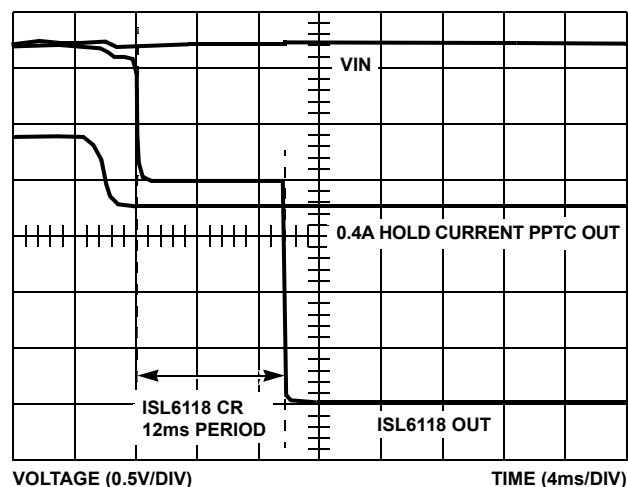
FIGURE 12. ISL6118 vs PPTC INTO 3.5Ω LOAD
