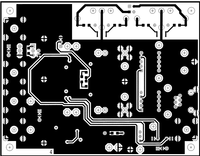
Figure 50. Layer 1
