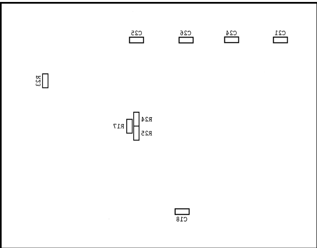
Figure 51. Silkscreen Bottom
