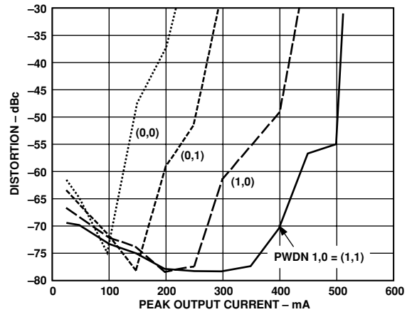
Figure 18. Distortion vs. Peak Output Current; Third Harmonic, V_S = \pm 6\text{ V} , G = +5 , R_L = 5\Omega , f = 100\text{ kHz} , Single-Ended
