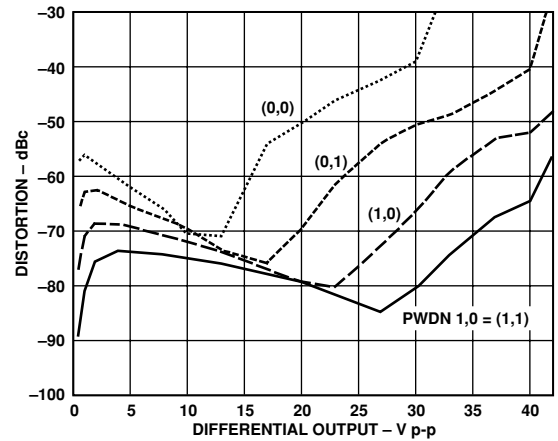
Figure 19. Distortion vs. Output Voltage; Third Harmonic, V_S = \pm 12\text{ V} , G = +10 , f = 1\text{ MHz} , R_L = 50\Omega , Differential
