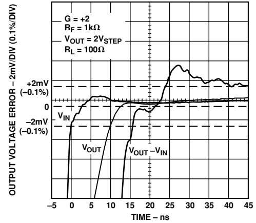
Figure 31. Settling Time 0.1%; V_S = \pm 6\text{ V}
