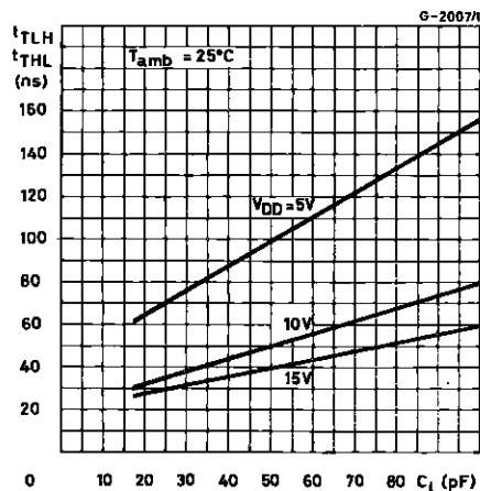
Typical Propagation Delay Time vs. Load Capacitance (Clock to Q1, 8 Bypass low).
