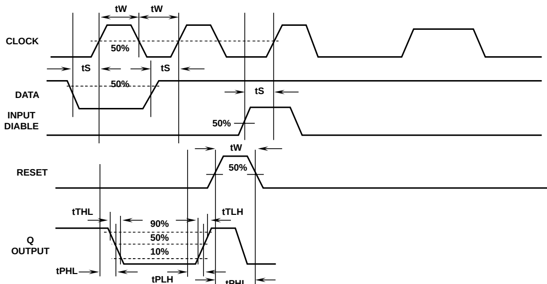
FIGURE 10. FUNCTIONAL WAVEFORM
