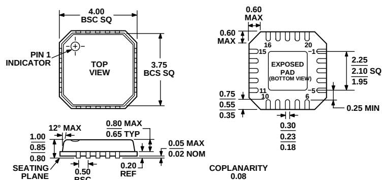
Figure 31. 20-Lead Lead Frame Chip Scale Package [LFCSP] 4 mm x 4 mm Body (CP-20-1) Dimensions shown in millimeters
