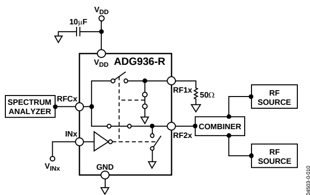
Figure 25. IP_3
