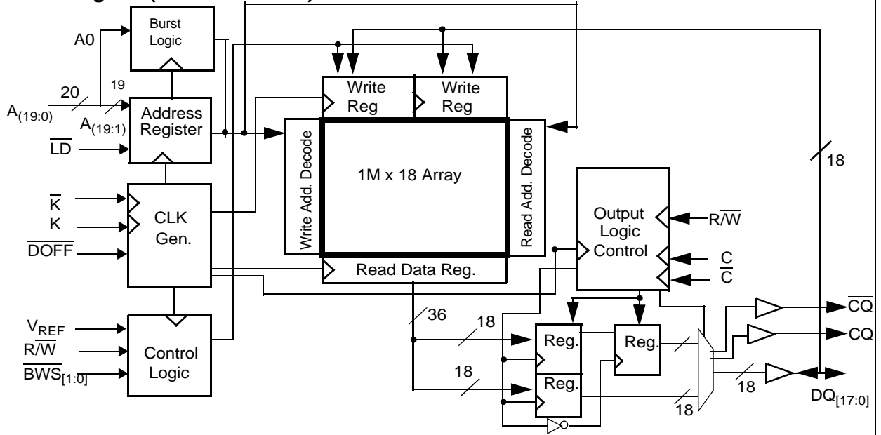
Logic Block Diagram (CY7C1318BV18)
