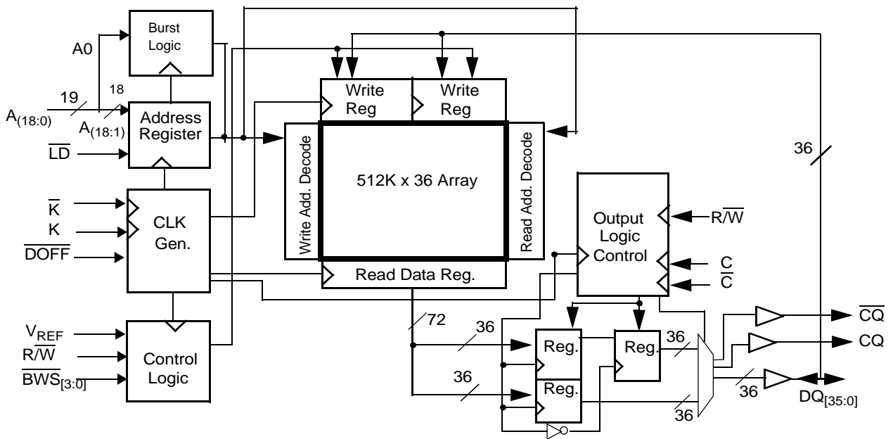
Logic Block Diagram (CY7C1320BV18)
