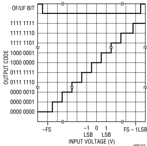
Figure 10. Transfer Characteristics
