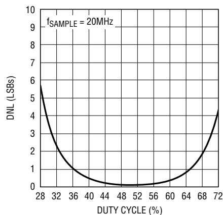
Figure 11. Typical DNL vs Duty Cycle
