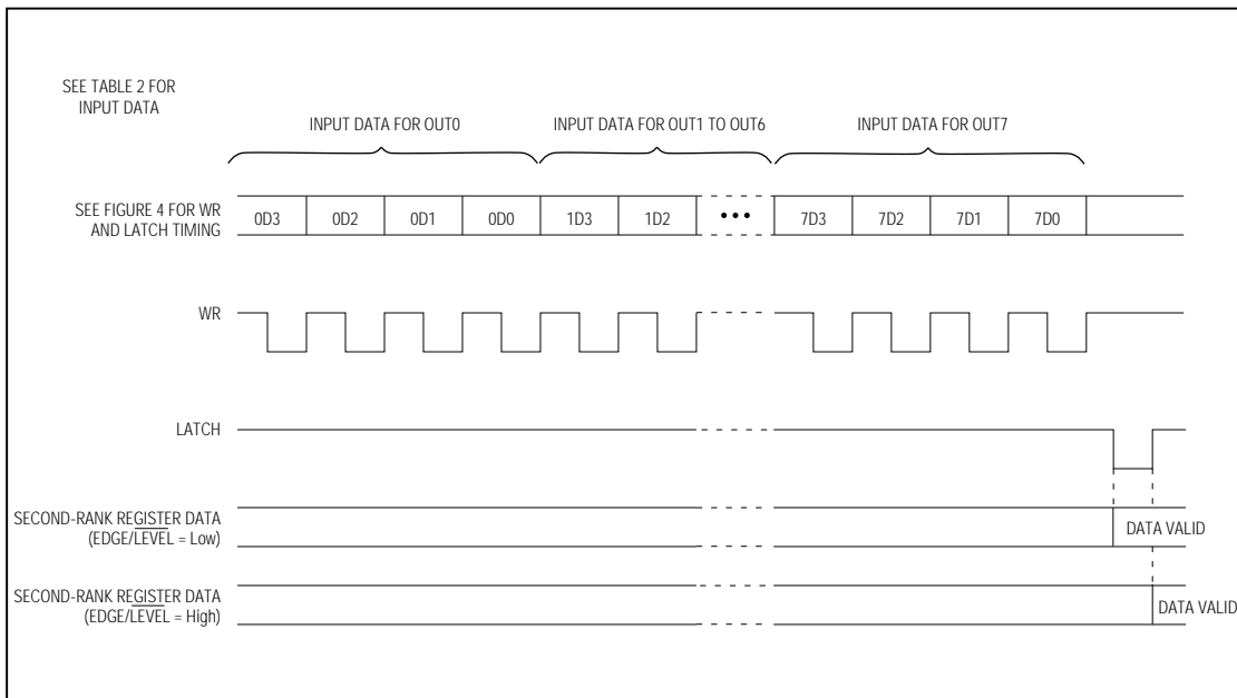
Figure 6. 32-Bit Serial-Mode Interface Format (SER/PAR = High)
