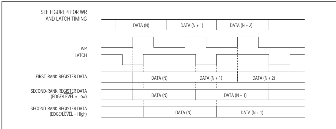
Figure 5. Parallel-Interface Mode Format (SER/PAR = Low)
