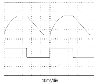
MAX866 SHUTDOWN RESPONSE (5V MODE)
