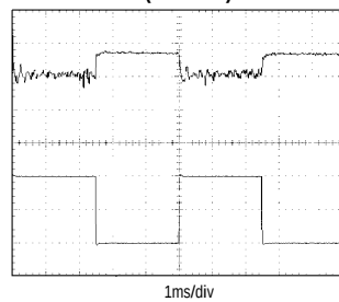
MAX866 LOAD-TRANSIENT RESPONSE (5V MODE)
