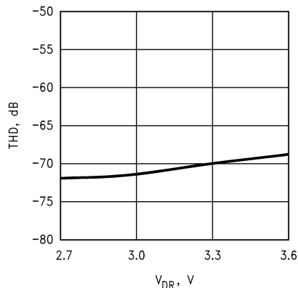
THD vs. V_{DR}
