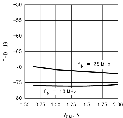
THD vs. V_{CM}
