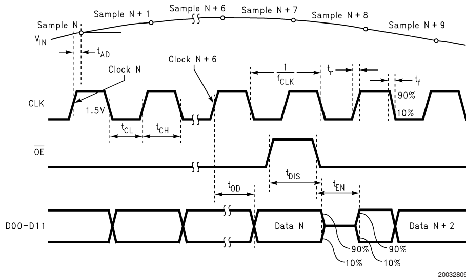
Output Timing
