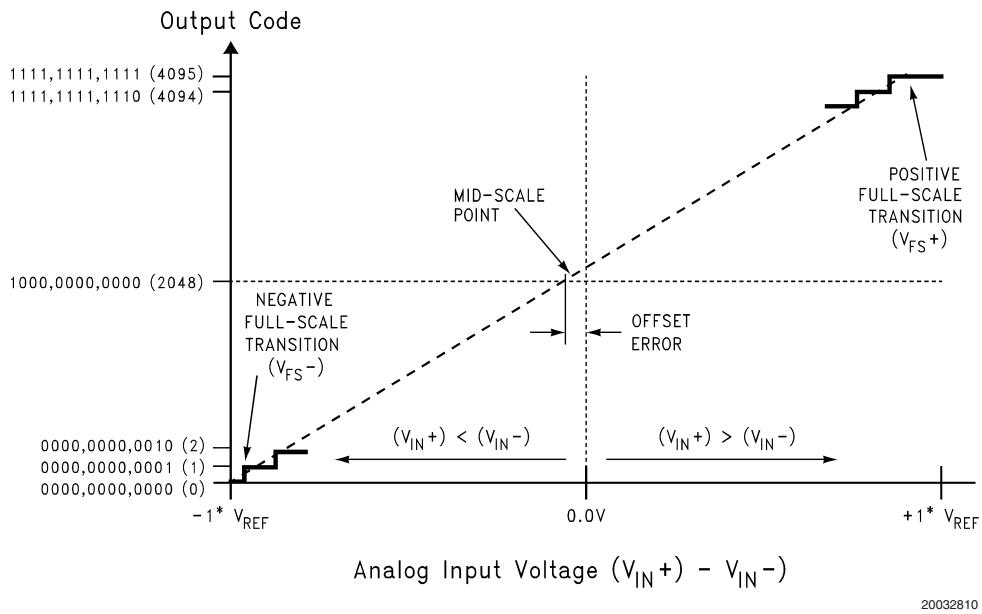
FIGURE 1. Transfer Characteristic
