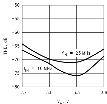
THD vs. V_A
