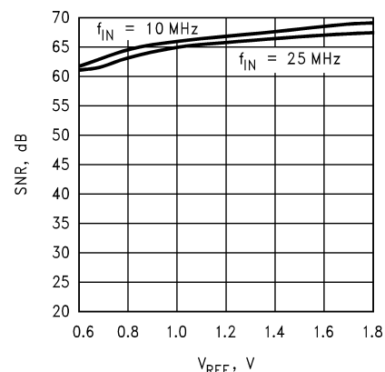
SNR vs. V_{REF}
