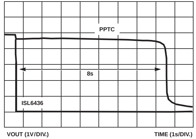
FIGURE 15. ISL6436 vs PPTC WITH EXTENDED 1.5A LOAD
