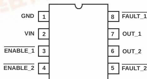
ISL6436 (SOIC) TOP VIEW
