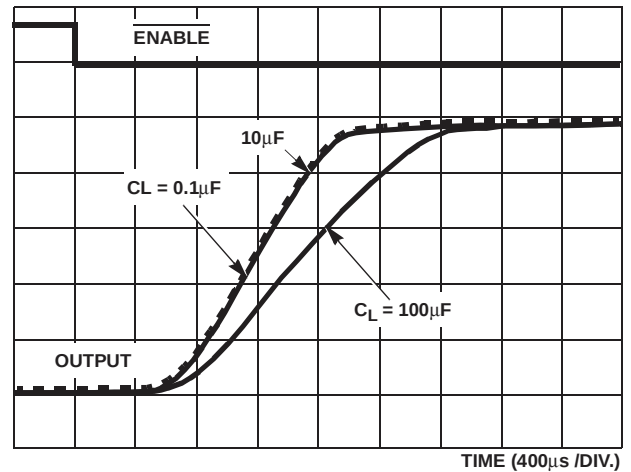
FIGURE 3. VOUT SOFT START vs C_{LOAD} , R_I \approx 10\Omega
