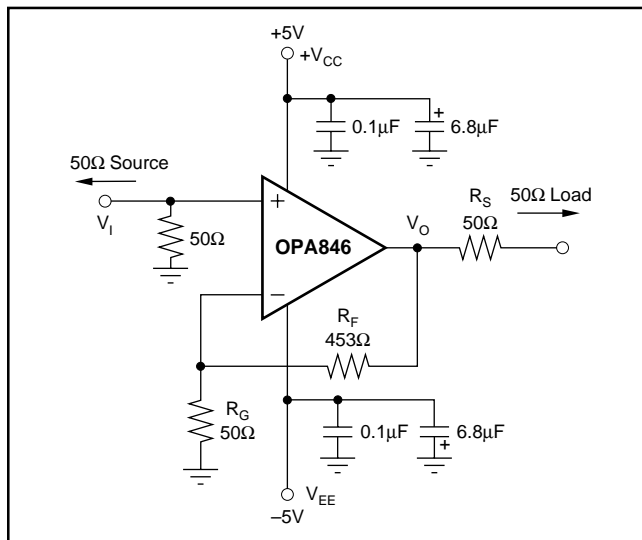
FIGURE 1. DC-Coupled, G = +10V/V , Bipolar Supply, Specification and Test Circuit.
