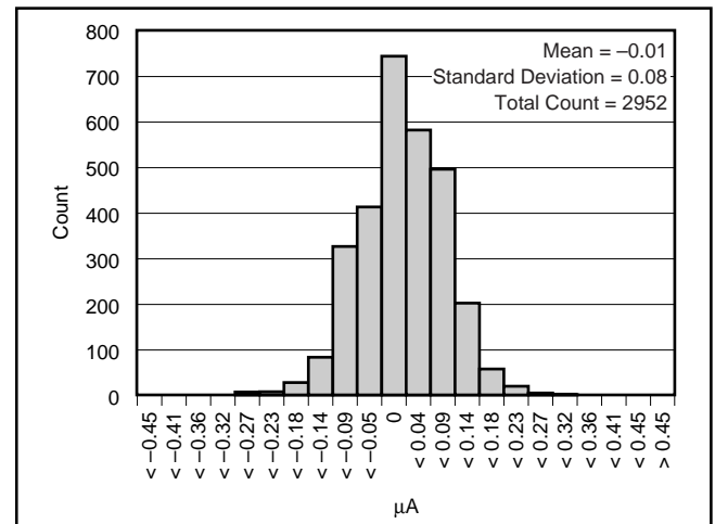
FIGURE 15. Input Offset Current Distribution.
