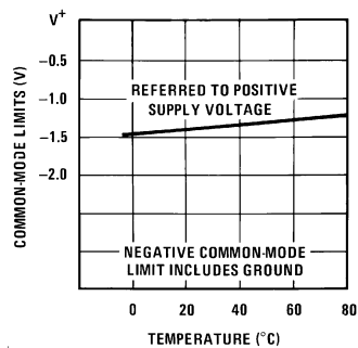
Common-Mode Limits
