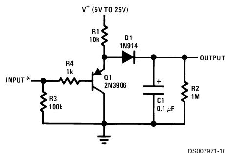
FIGURE 3. Half-Wave Peak Detector
