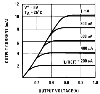
Output Characteristics
