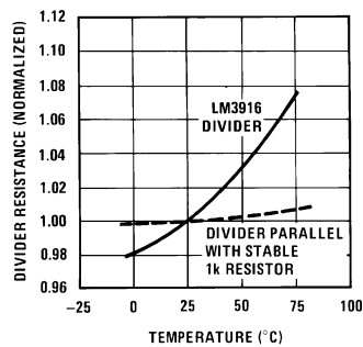
Total Divider Resistance vs Temperature
