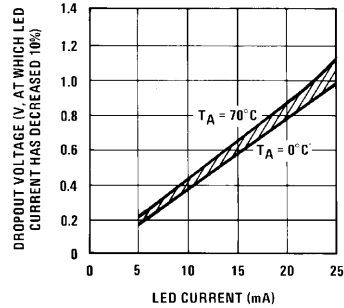
LED Current-Regulation Dropout
