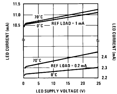
LED Driver Current Regulation
