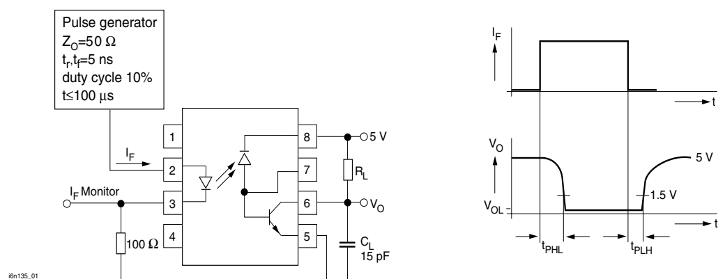
Figure 1. Switching Times
