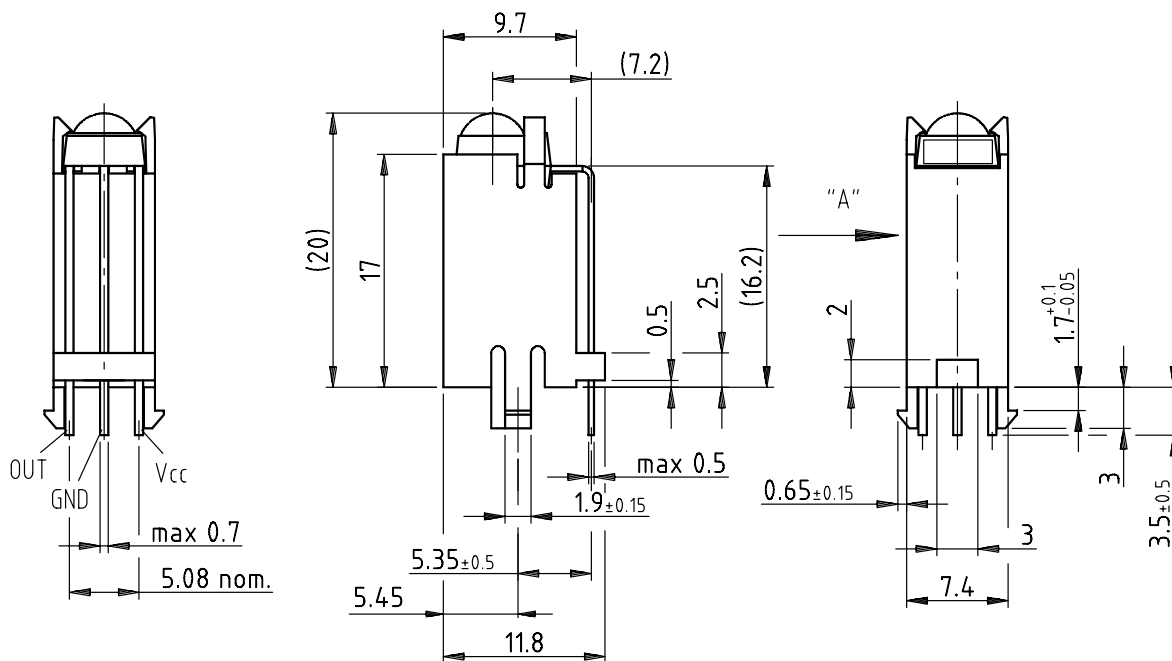
View "A"
