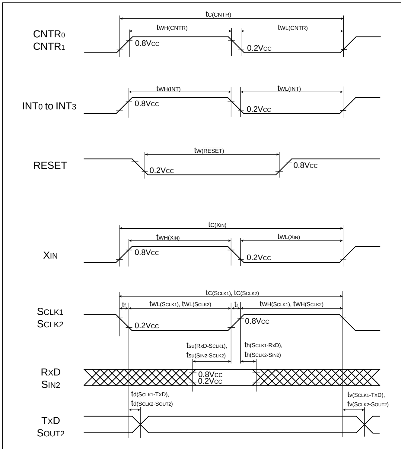
Fig. 77 Timing diagram
