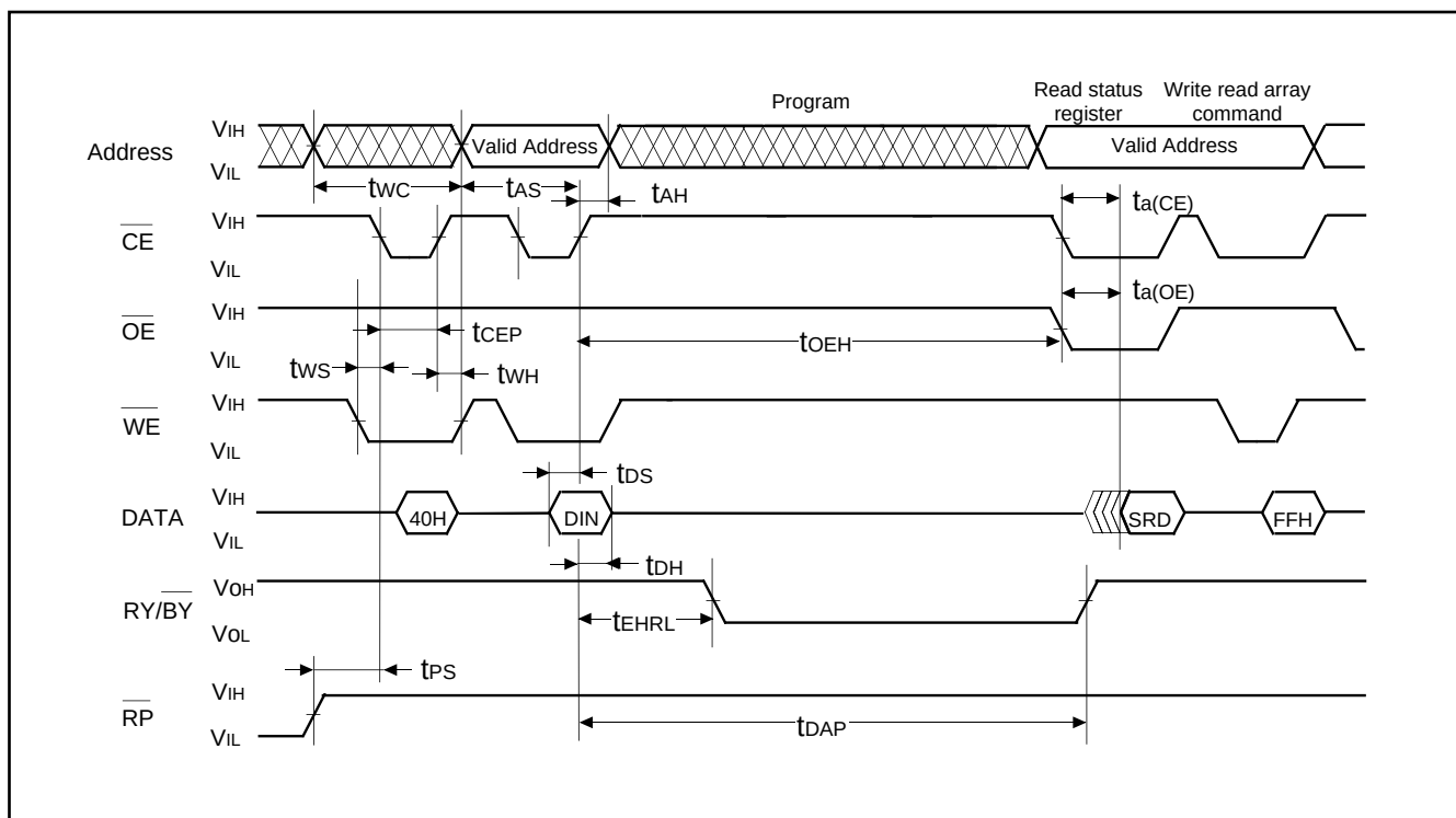
Fig. 70 AC wave for program operation (CE control)
