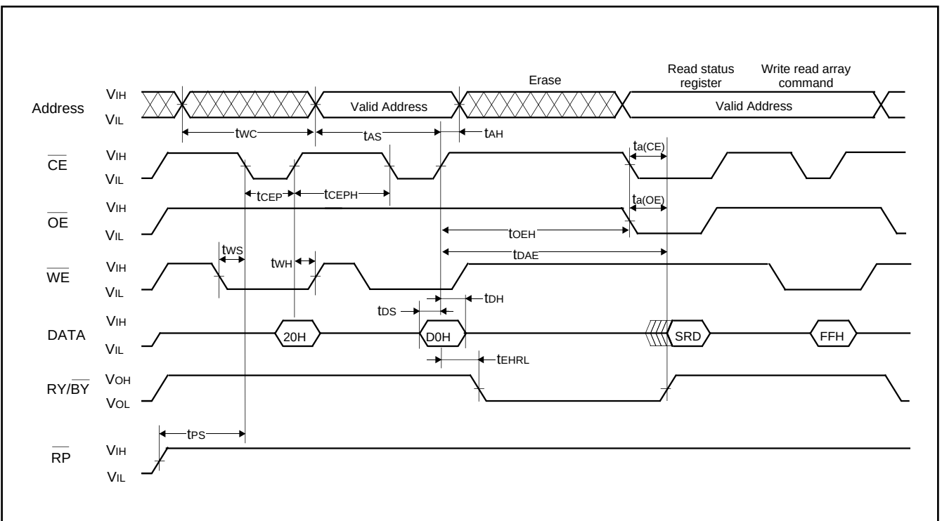
Fig. 74 AC wave for erase operation ( \overline{\text{CE}} control)
