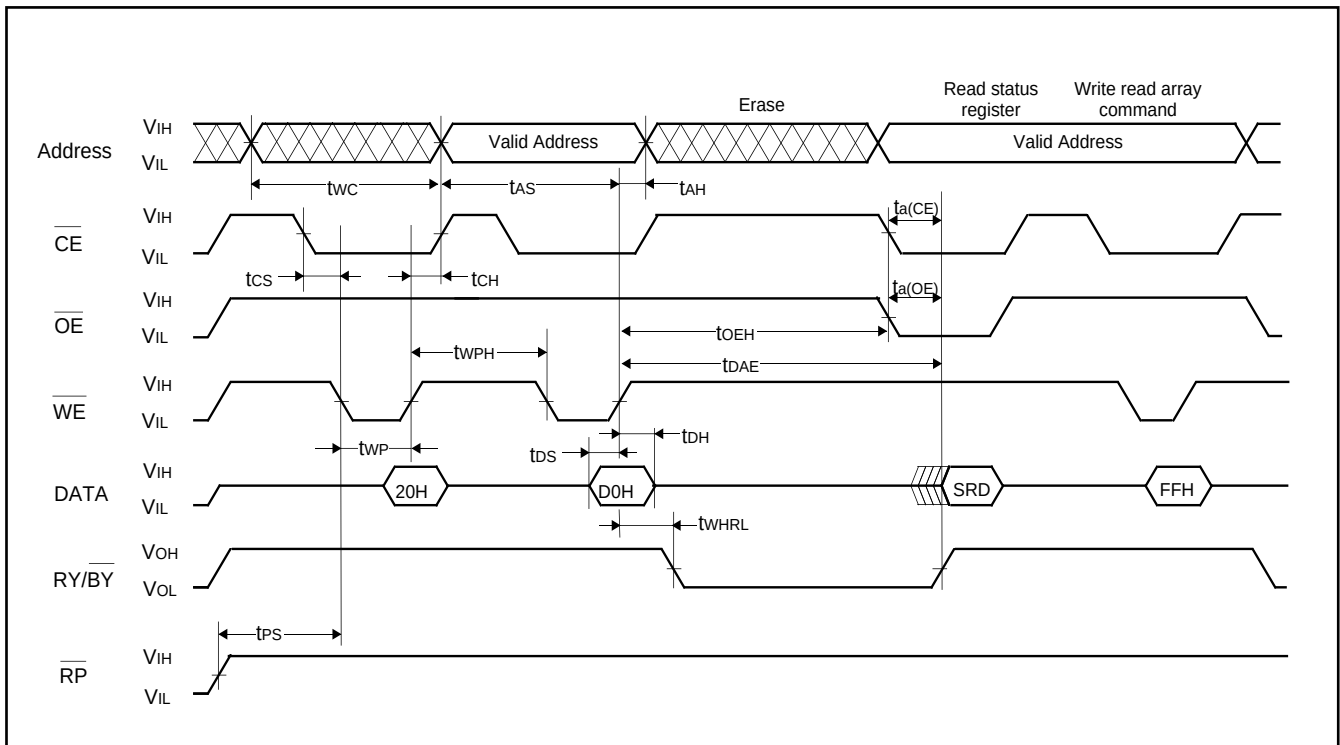
Fig. 73 AC wave for erase operation ( \overline{\text{WE}} control)
