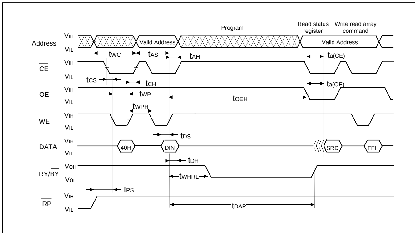
Fig. 69 AC wave for program operation (WE control)
