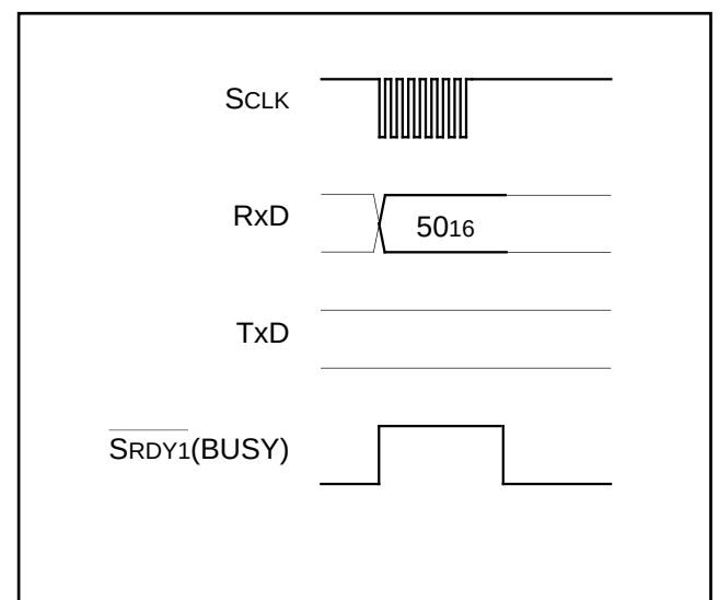
Fig. 59 Timing for clearing the status register
