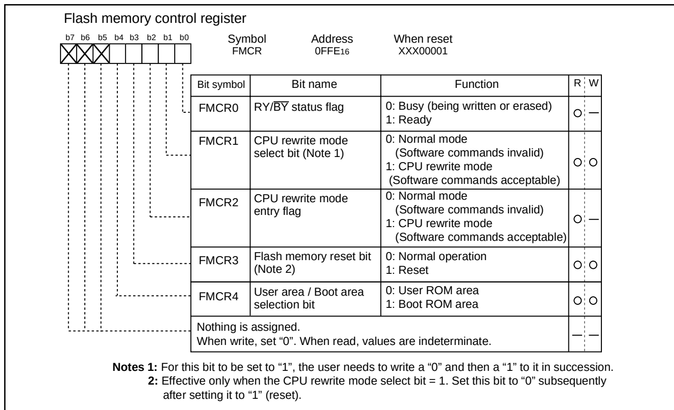
Fig. 45 Flash memory control registers
