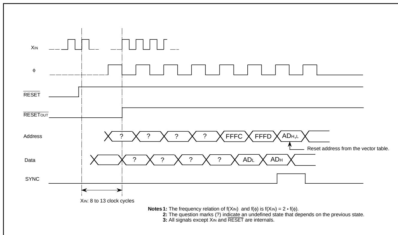
Fig. 37 Reset sequence
