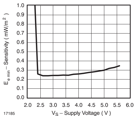
Figure 12. Sensitivity vs. Supply Voltage
