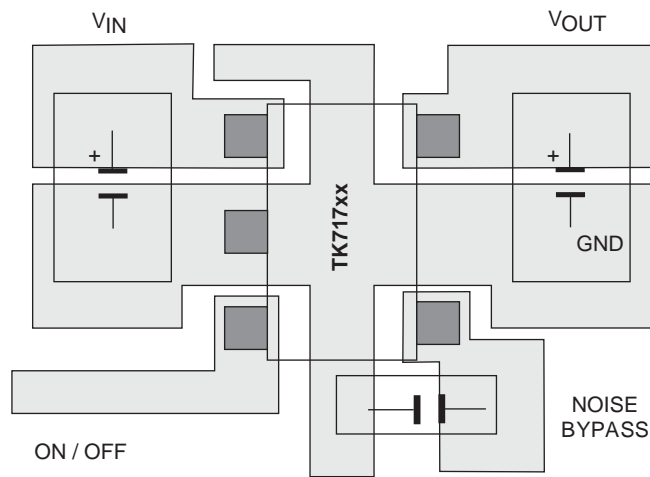
SOT23-5 BOARDLAYOUT
