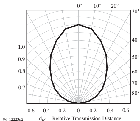
Figure 13. Directivity
