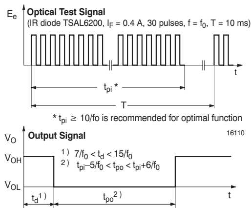
Figure 1. Output Function
