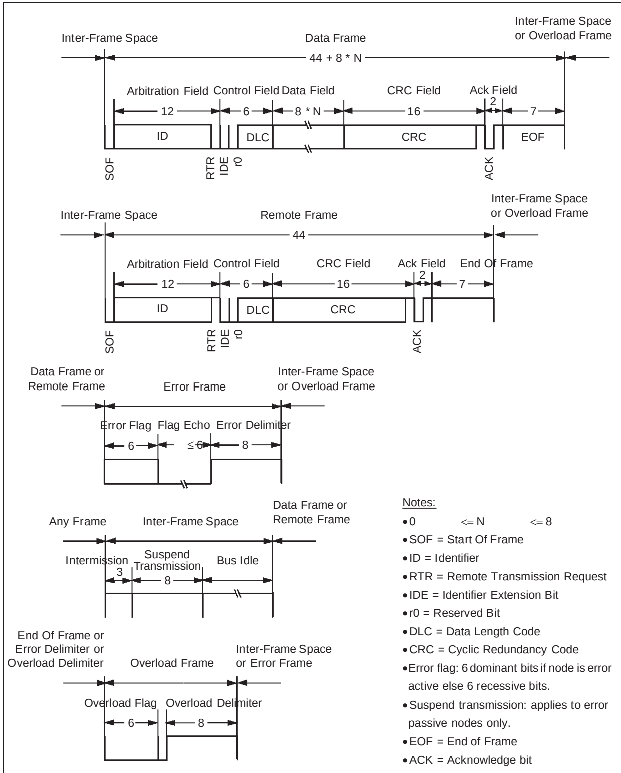
Figure 56. CAN Frames
