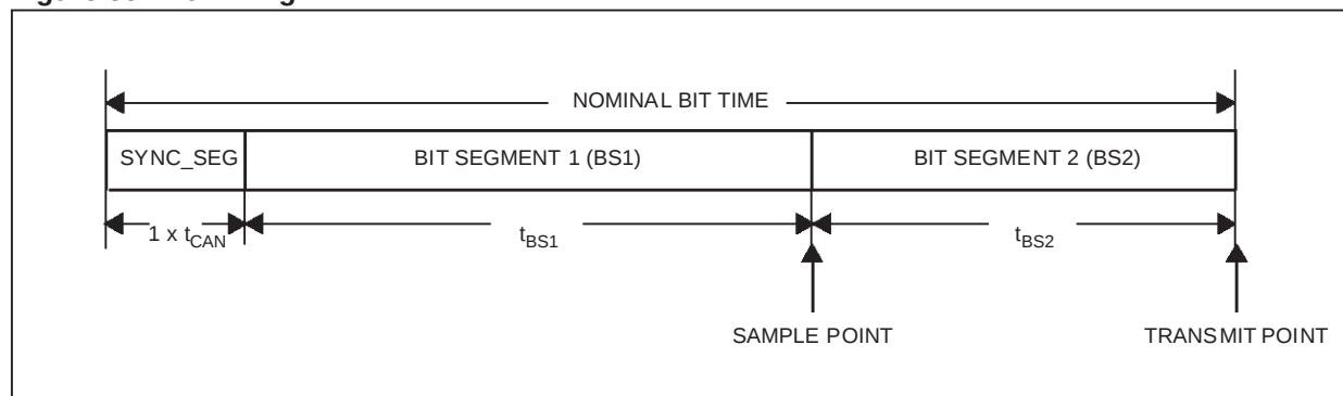
Figure 59. Bit Timing
