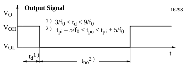
Figure 7. Output Function
