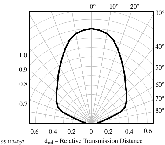
Figure 14. Horizontal Directivity \varphi_x
