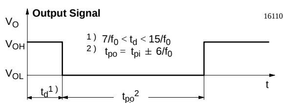
Figure 7. Output Function
