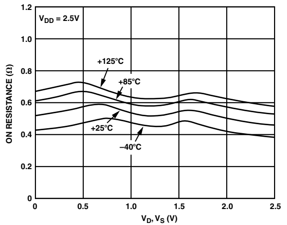
TPC 5. On Resistance vs. V_D ( V_S ) for Different Temperature, 2.5 V
