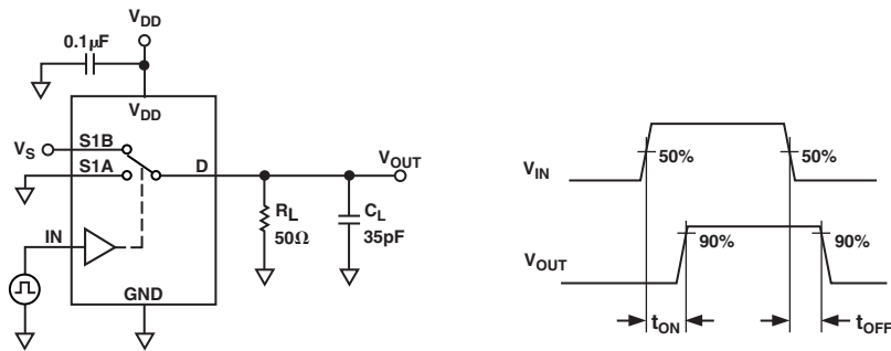
Test Circuit 4. Switching Times, t_{ON} , t_{OFF}
