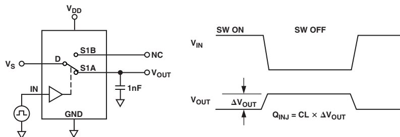
Test Circuit 6. Charge Injection
