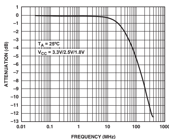
TPC 12. Bandwidth
