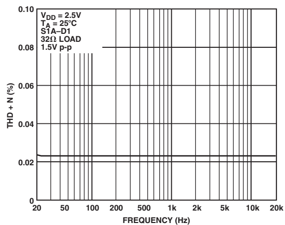
TPC 15. Total Harmonic Distortion + Noise
