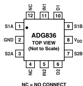
12-Lead LFCSP (CP-12)
