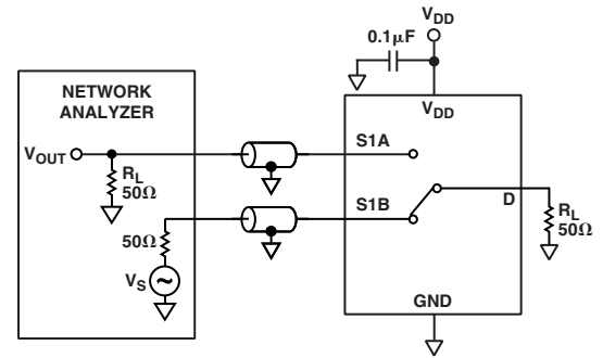
Test Circuit 9. Channel-to-Channel Crosstalk (S1A-S1B)
